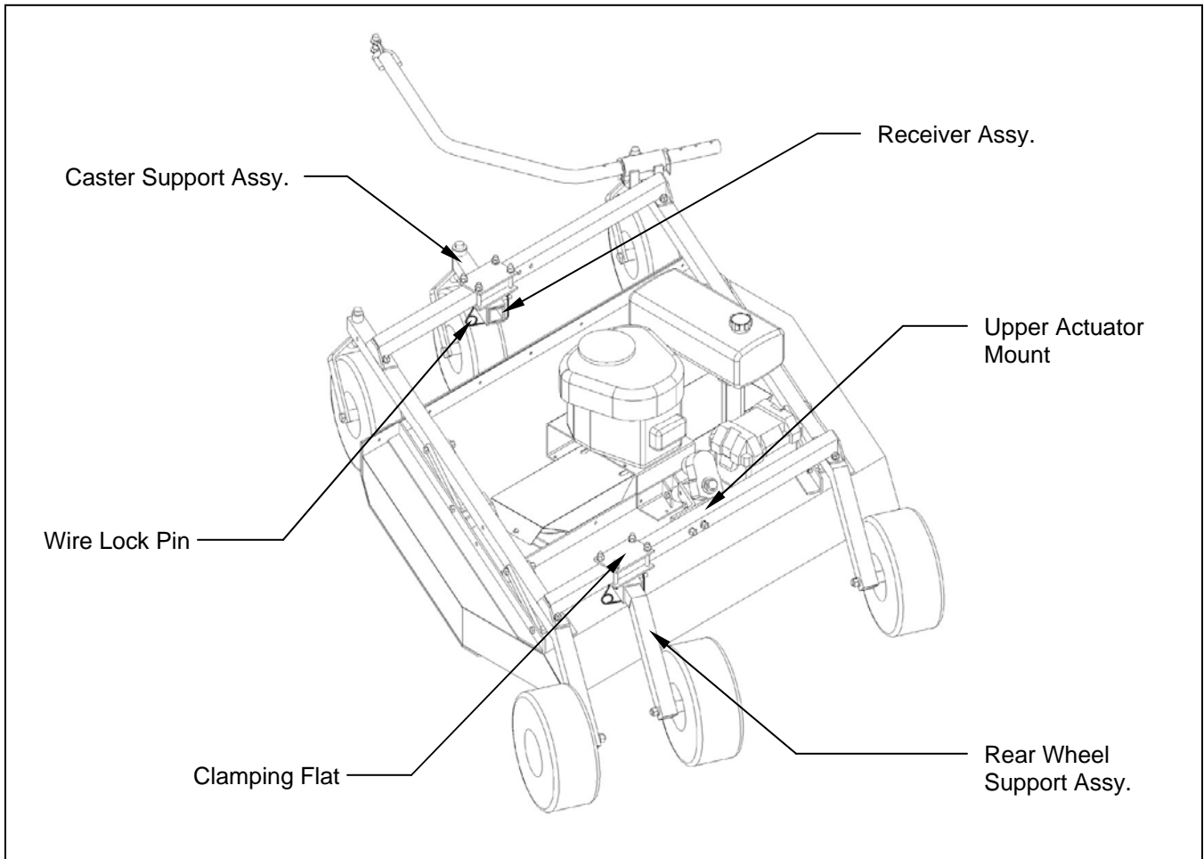
Figure 3. Assembly of Floatation Kit Parts on Electric Lift Kit Models
